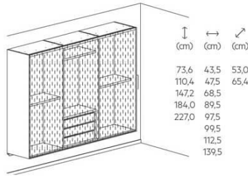
Struttura a vani sospesi Wall-mounted compartment structure
